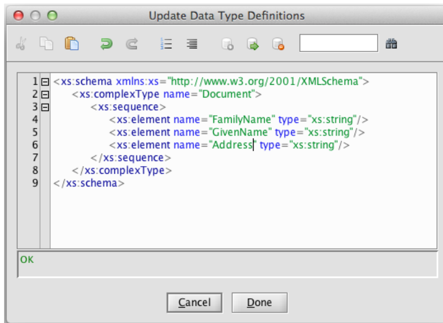
Figure 9.11: Data Definition for 'Document' type
