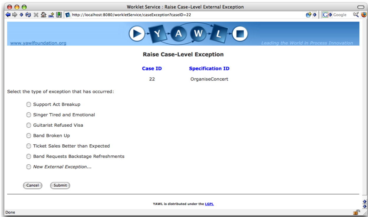
Figure 8.40: Raise Case-Level Exception Screen (Organise Concert example)
