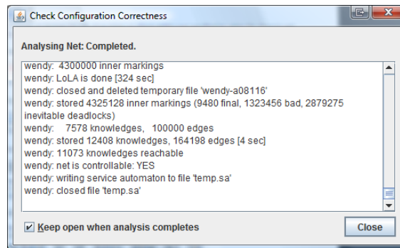
Figure 4.69: Output from Wendy.
