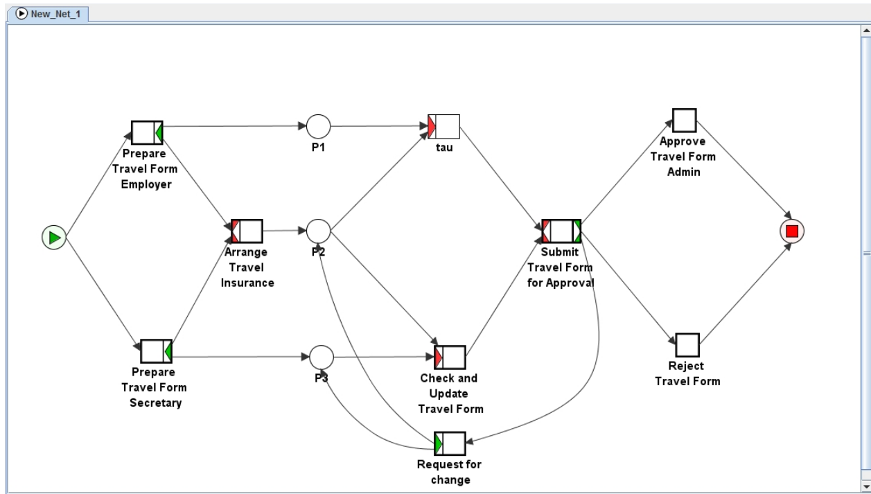
Figure 4.65: A C-YAWL model for travel requisition
