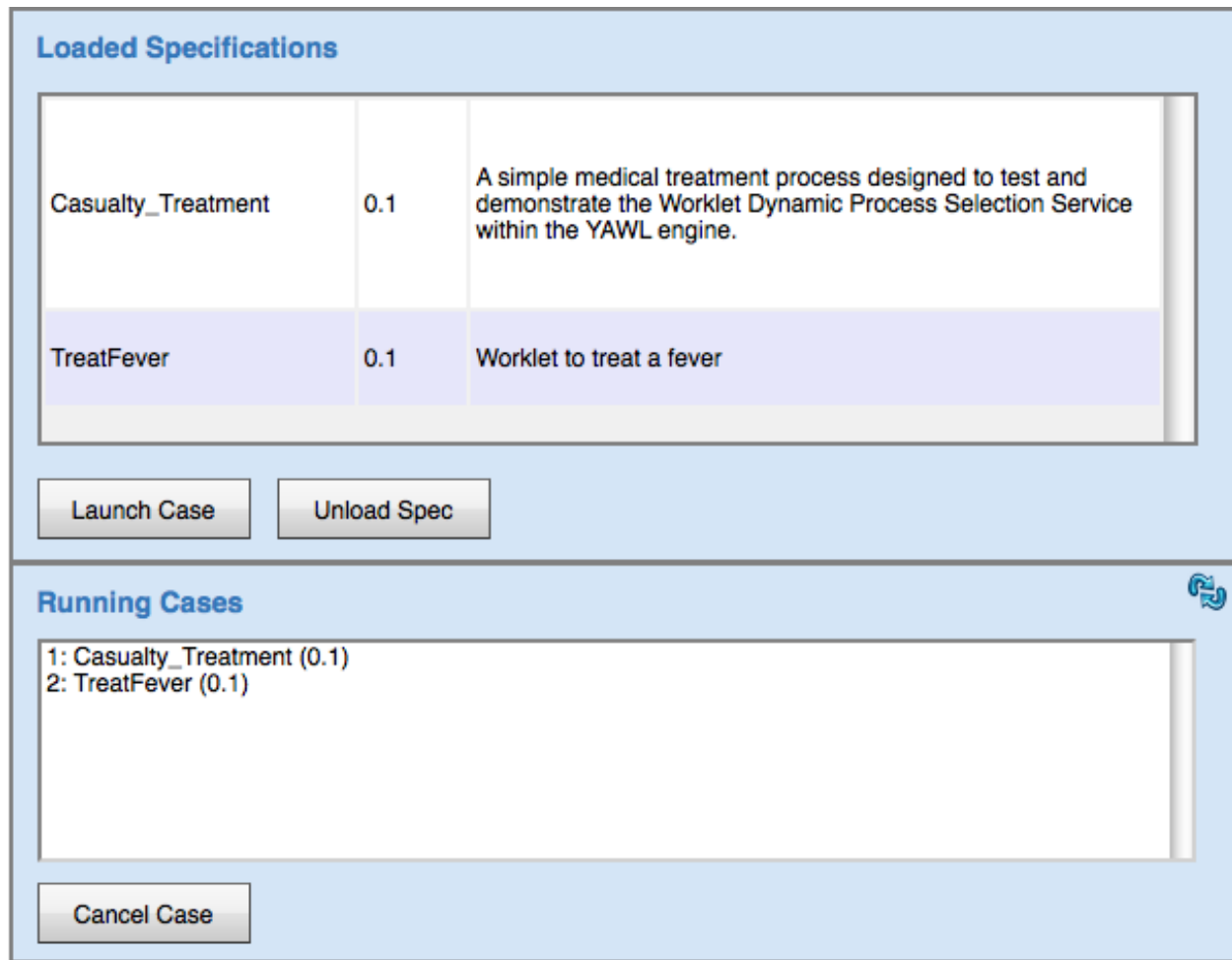
Figure 8.25: TreatFever Specification Uploaded and Launched
