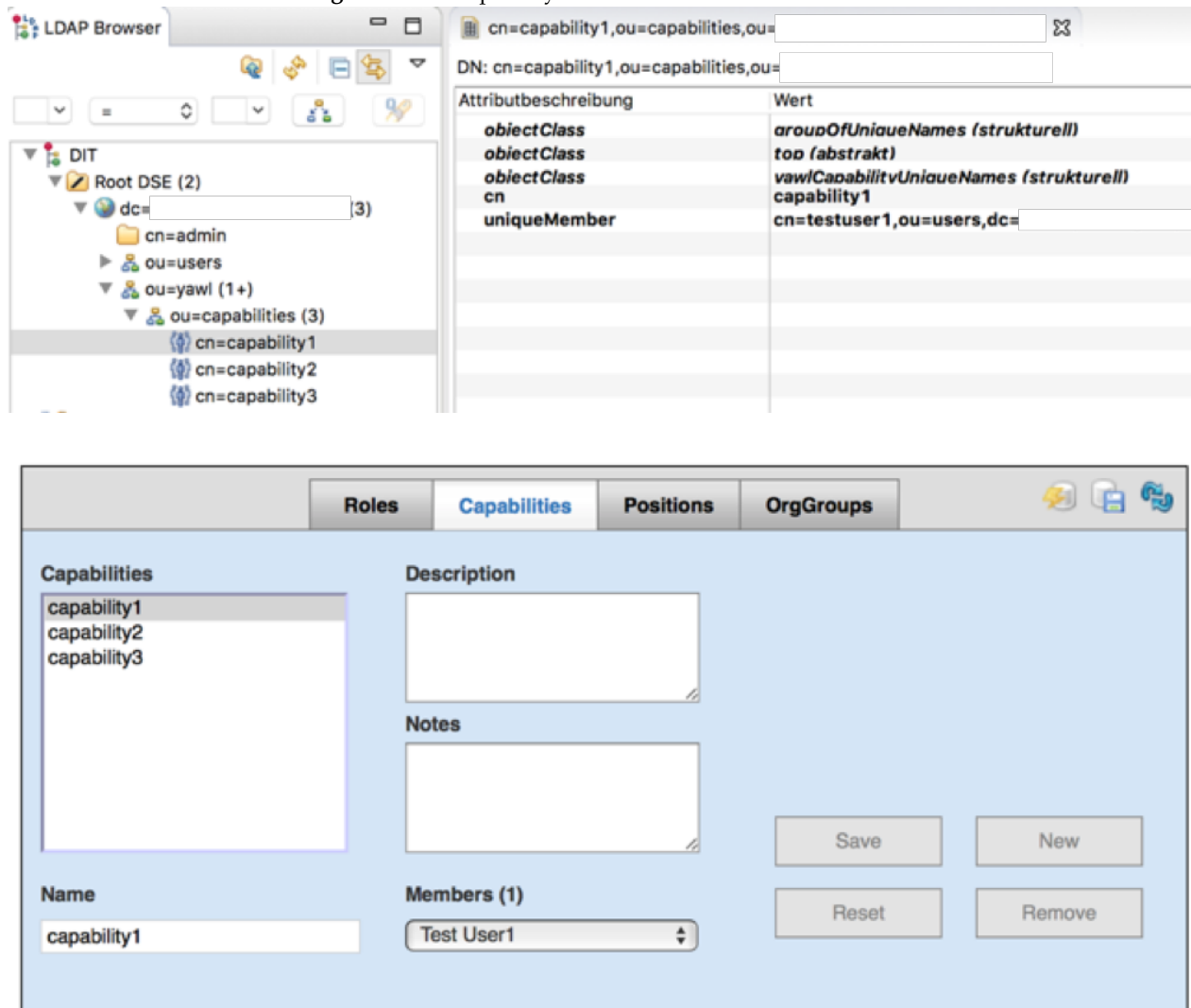
Figure 10.4: A capability modelled in LDAP and in YAWL
