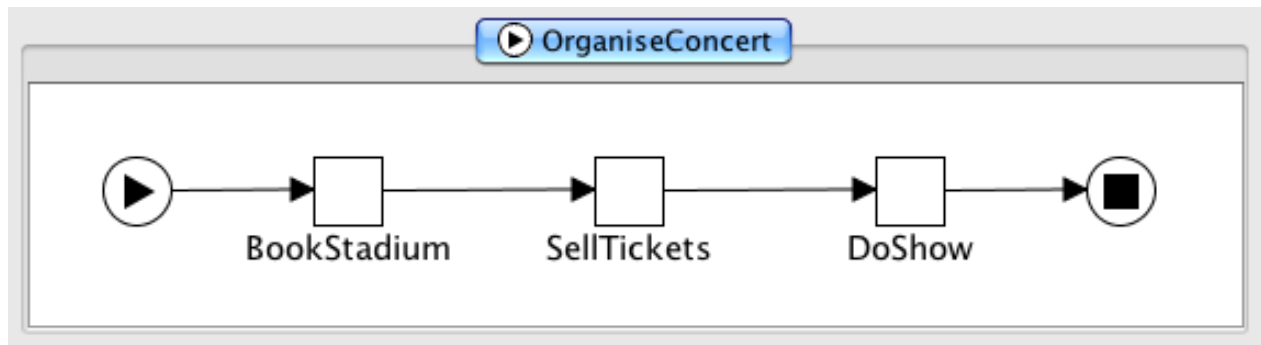
Figure 8.34: The OrganiseConcert Specification
