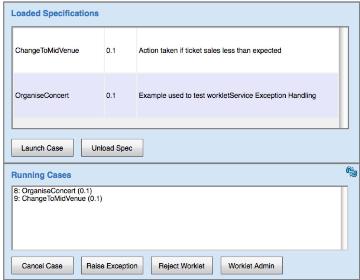
Figure 8.39: Case Mgt Screen, OrganiseConcert case running
