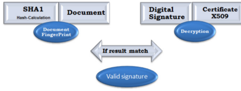
Figure 9.5: An overview of the verification of a digital signature
