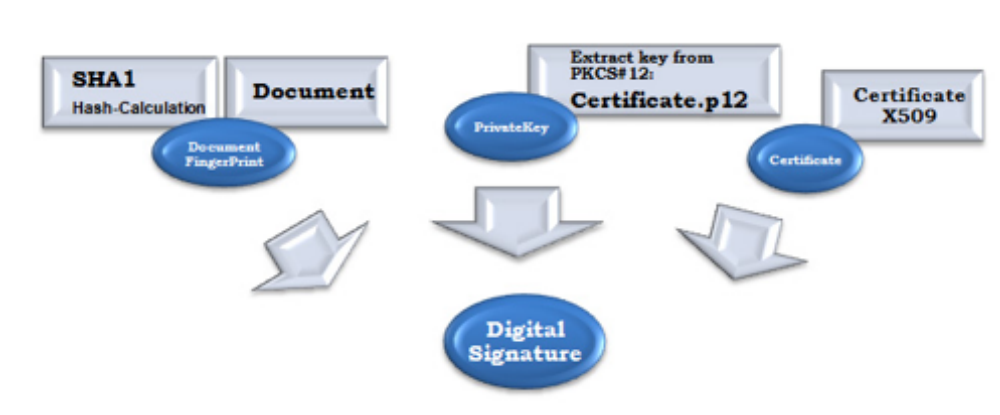
Figure 9.4: An overview of the production of a digital signature
