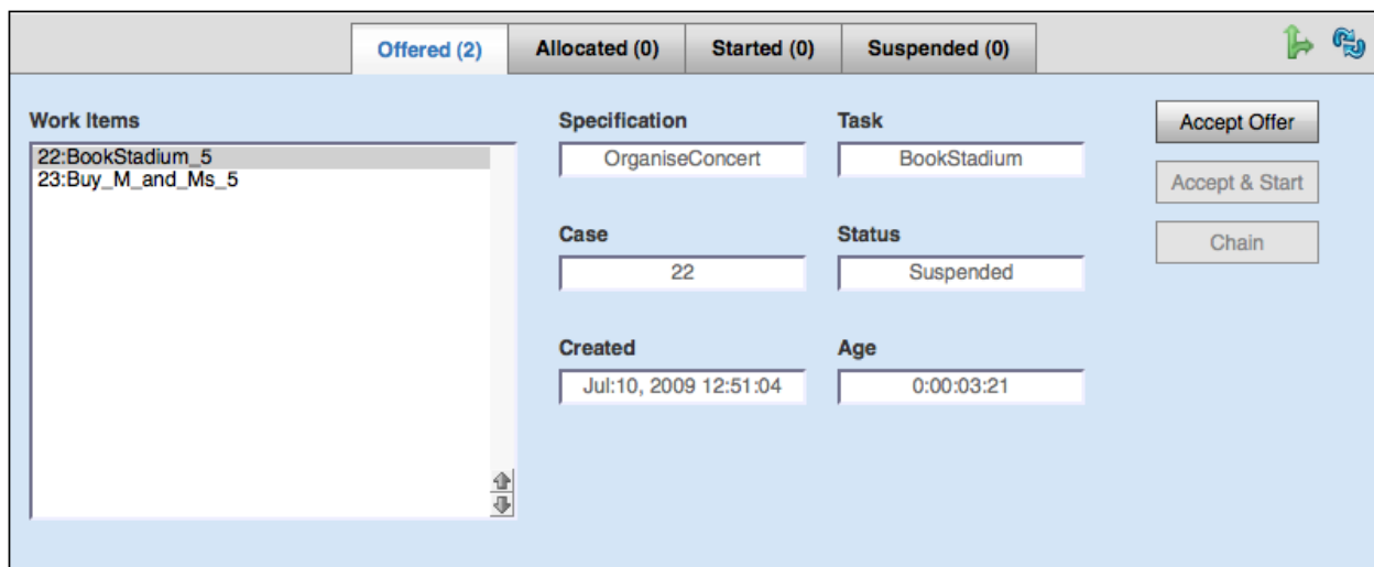
Figure 8.41: Available Work Items after External Exception Raised
