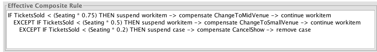
Figure 8.37: Effective Composite Rule for Do Shows Pre-Item Constraint Tree
