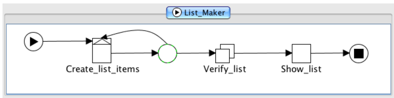
Figure 8.29: The wListMaker Specification
