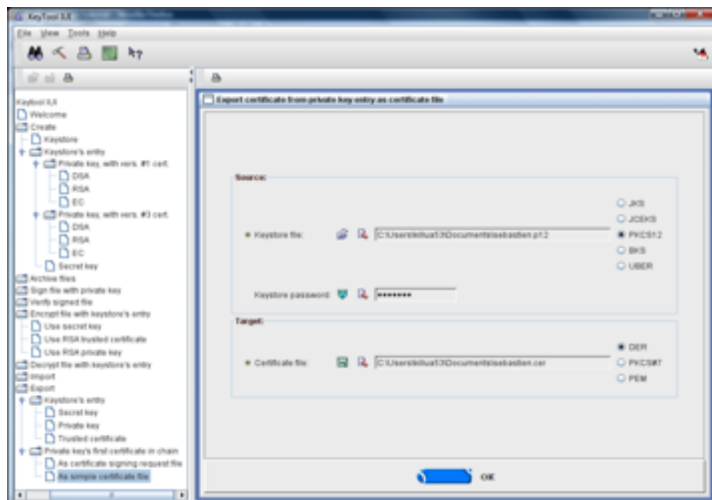
Figure 9.9: Exporting the Certificate
