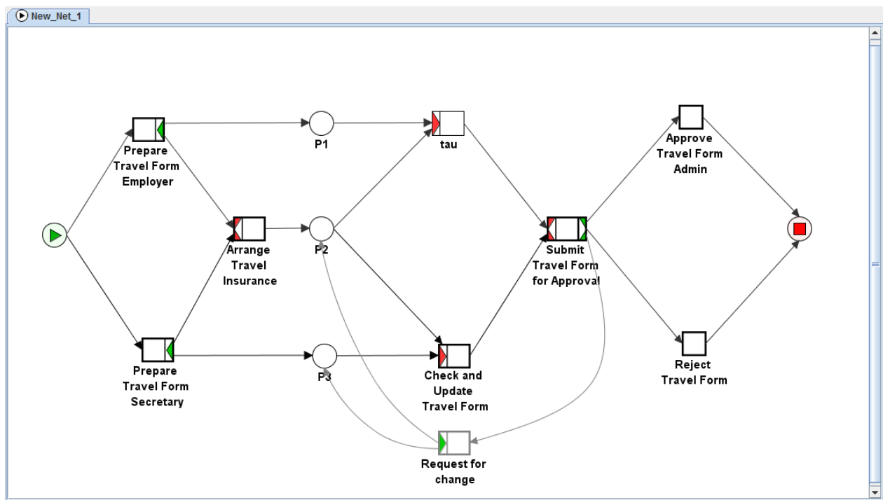
Figure 4.67: The preview of a process model configuration.
