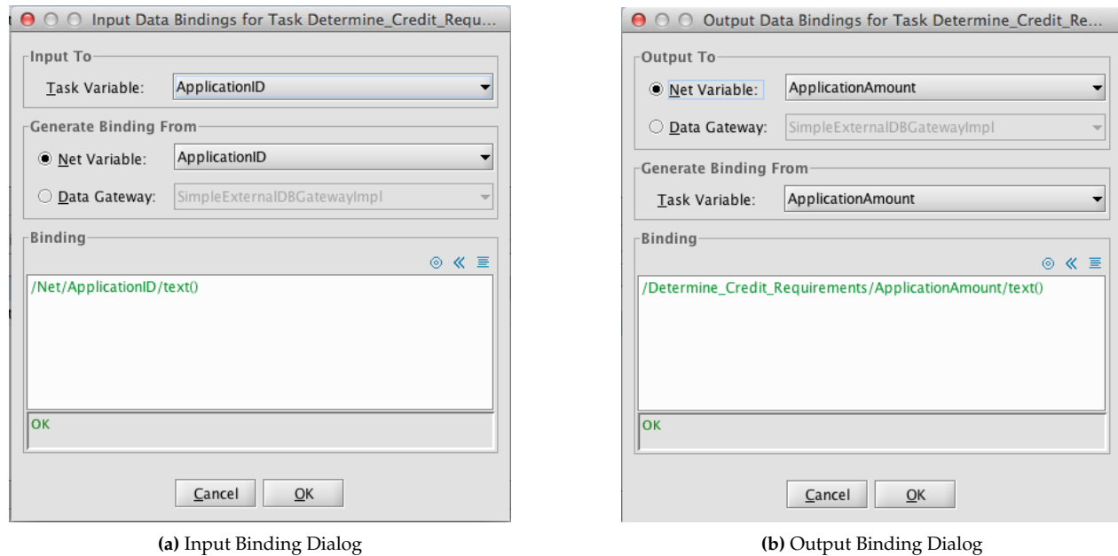
Figure 3.12: Data Mappings for Determine Credit Requirements Variables
