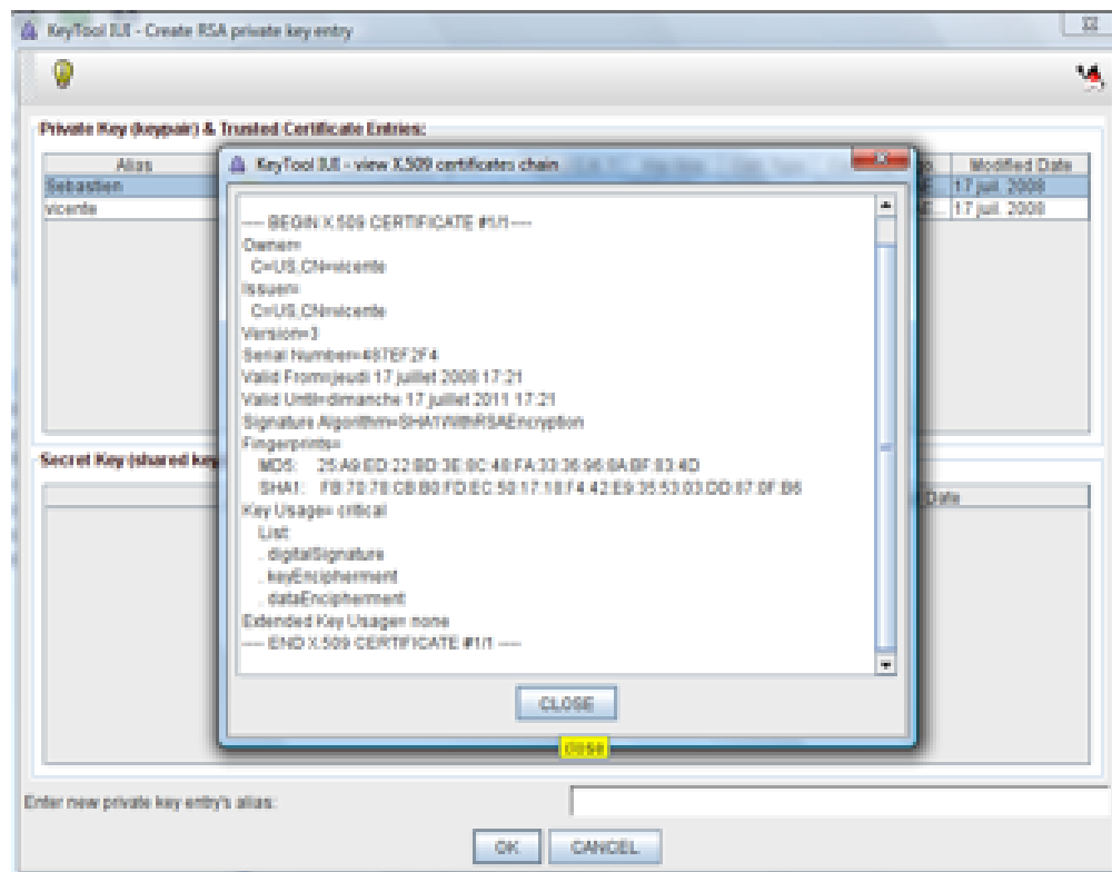
Figure 9.8: The Created Certificate
