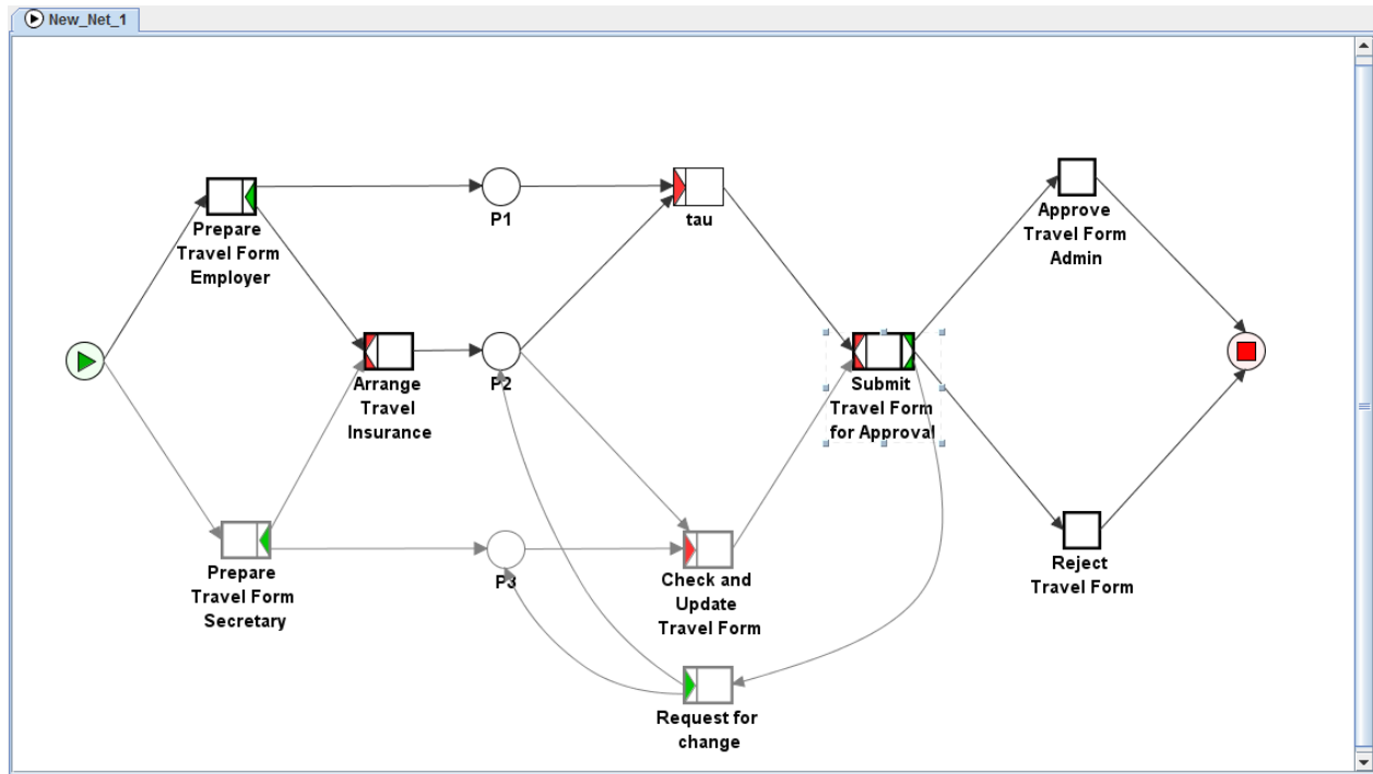
Figure 4.70: Preview of the configuration after blocking the input port of task “Check and Update Travel Form”
