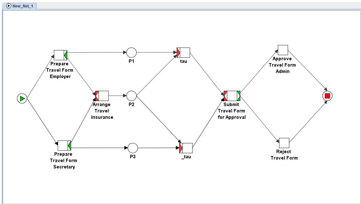
Figure 4.68: The result of committing a process model configuration.
