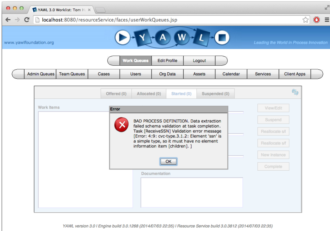
Figure 5.11: An error indicating invalid semantics of an XQuery used in the specification
